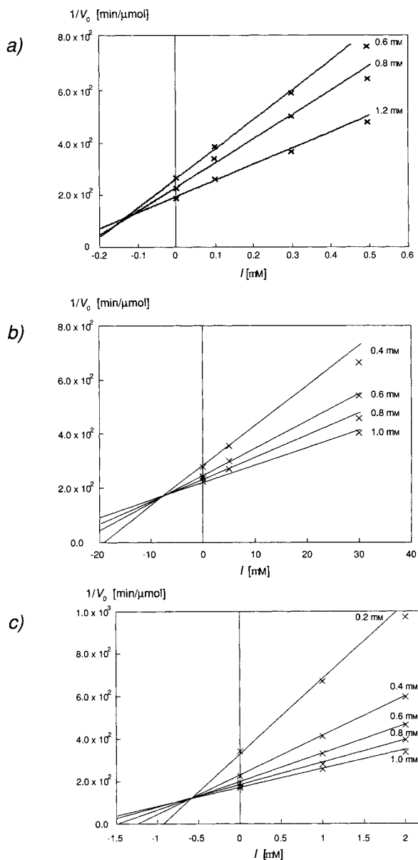
Fig. 3. Dixon plot for inhibition of a) bovine, b) Aspergillus , and c) Artemia N-acetylglucosaminidase by 4
