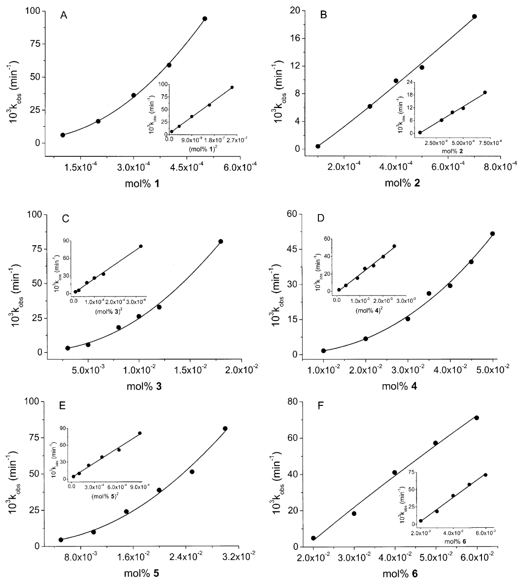
Figure 1. Plots of k_{\text{obsd}} versus (mol % conjugate) for (A) 1, (B) 2, (C) 3, (D) 4, (E) 5, and (F) 6 in POPC liposomes at 35 °C. The solid lines are nonlinear least-squares fit of the data according to k_{\text{obsd}} = k_0 + k_2(\text{mol \% conjugate})^n/K , where n = 2.0, 1.1, 2.1, 2.2, 2.0 , and 0.9 , respectively; insets represent similar plots where n has been fixed at 2.0, 1.0, 2.0, 2.0, 2.0, and 1.0 for 1, 2, 3, 4, 5, and 6, respectively.
