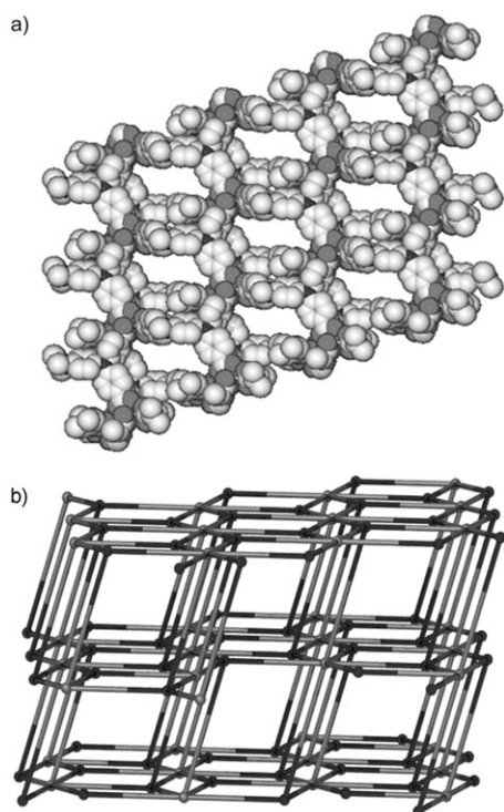
Figure 4. a) The three-dimensional porous framework of 3 viewed along the b axis. b) A schematic representation of 3 simplifying the organic ligand as a pseudotetrahedral connector and the hourglass SBU as an eight-connected node.
