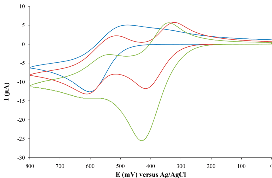
FIGURE 6. Cyclic voltammograms (0.1 M [Bu 4 N]ClO 4 , CH 3 CN, 100 mV/s) of 4 (blue line), 4 + 0.5 equiv of [Bu 4 N]C 6 H 5 COO (red line), and 4 + 1.0 equiv of [Bu 4 N]C 6 H 5 COO (green line).
