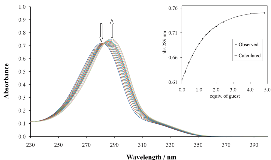
FIGURE 3. Family of UV-vis spectra taken in the course of the titration of a 1.75 \times 10^{-5} M solution of 2 in \text{CH}_3\text{CN} with a standard solution of [\text{Bu}_4\text{N}]\text{CH}_3\text{COO} . Inset shows the titration profile from which the association constant was determined, \log K = 4.4 \text{ M}^{-1} .
