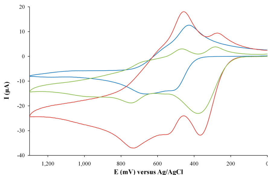
FIGURE 5. Cyclic voltammograms (0.1 M [Bu 4 N]ClO 4 , CH 3 CN, 100 mV/s) of 2 (blue line), 2 + 0.5 equiv of [Bu 4 N]C 6 H 5 COO (red line), and 2 + 1.0 equiv of [Bu 4 N]C 6 H 5 COO (green line).
