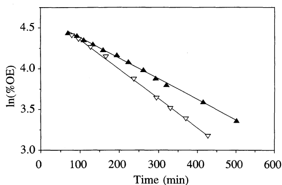
Fig. 3. Hydrolysis of DETOSU-CDM ( \nabla ) and DETOSU-HD ( \blacktriangle ) in p -dioxane- d_8 containing \text{D}_2\text{O} (2.01 M) at 37^\circ\text{C} , reaction catalyzed by 2.0 mM of dichloroacetic acid. Data obtained by ^1\text{H} NMR.
