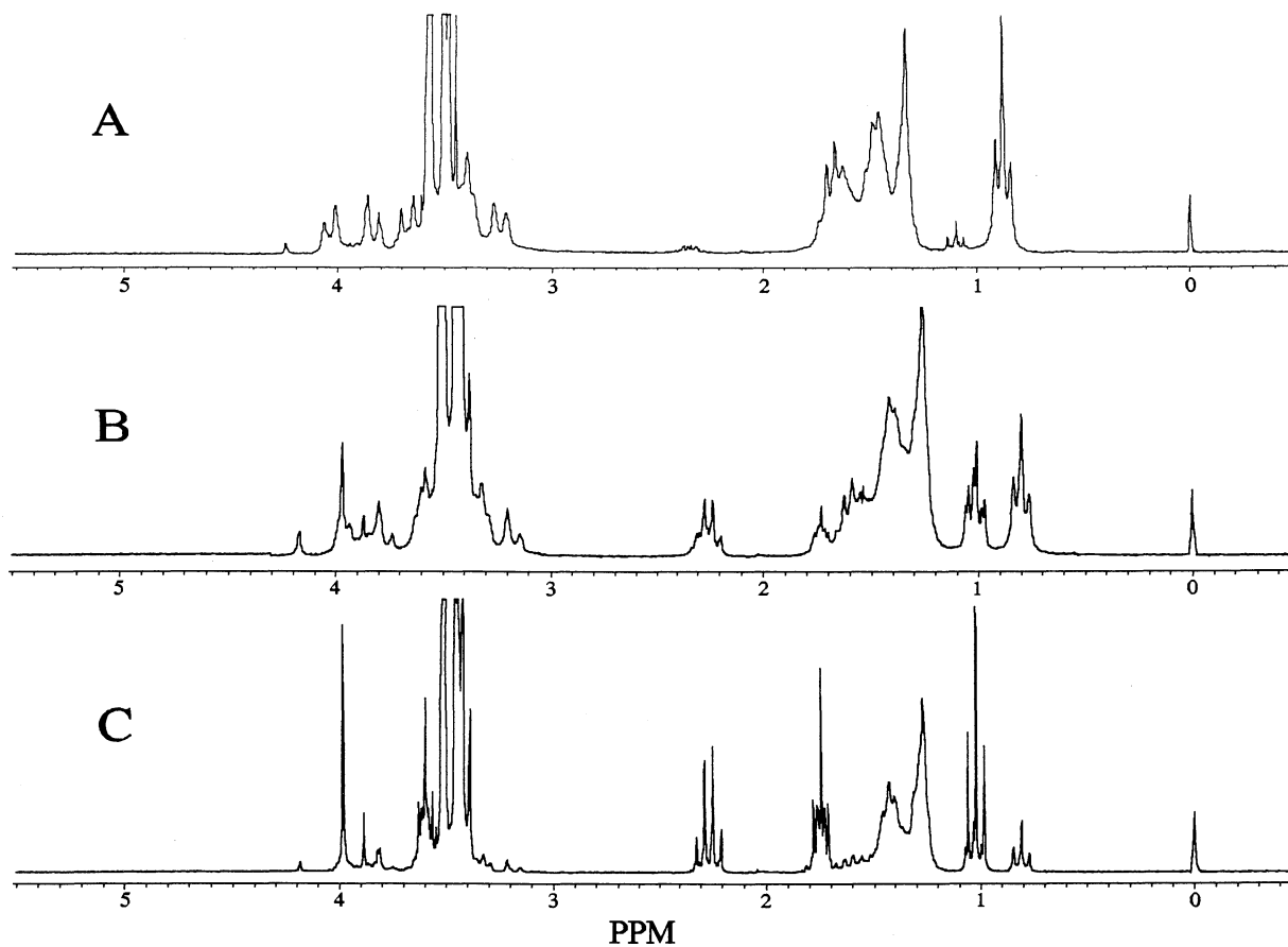
Fig. 1. ^1\text{H} NMR spectra of DETOSU-HD in p-dioxane- \text{d}_8 containing 2.01 M of \text{D}_2\text{O} and 2 mM dichloroacetic acid ( 37^\circ\text{C} ). Spectra taken when 95% (A), 59% (B) and 18% (C) of the ortho ester bonds remained.
