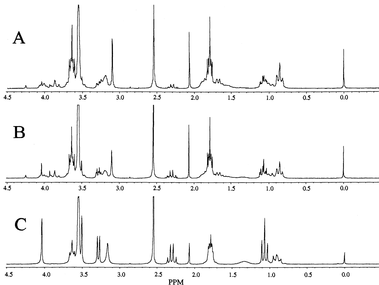
Fig. 2. ^1\text{H} NMR spectra of DETOSU-CDM taken when 26% (A), 33% (B), and 74% (C) of the backbone ortho ester bonds were hydrolyzed at 37^\circ\text{C} in p -dioxane- d_8 containing \text{D}_2\text{O} (2.01 M). Hydrolysis was catalyzed by 2.0 mM of dichloroacetic acid.
