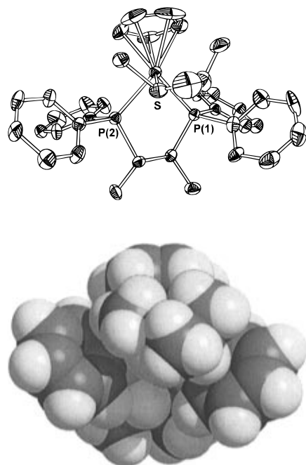
Figure 2. Ortep plot and space-filling model of the cation [\text{CpRu}(\text{chir})(\text{MeS-}i\text{-Pr})]^+ ( 5b + ).
