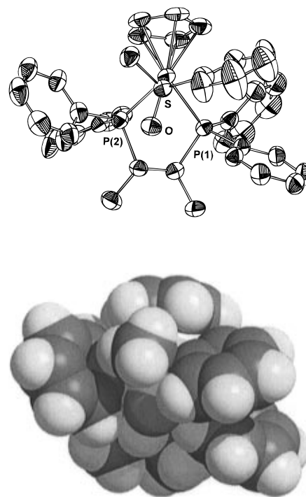
Figure 3. Ortep plot and space-filling model of the cation [\text{CpRu}(\text{chir})(\text{MeS}(\text{O})\text{Ph})]^+ ( 10a + ).
