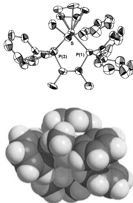
Figure 1. Ortep plot and space-filling model of the cation [CpRu(chir)(MeSPh)]⁺ ( 5a ⁺).
