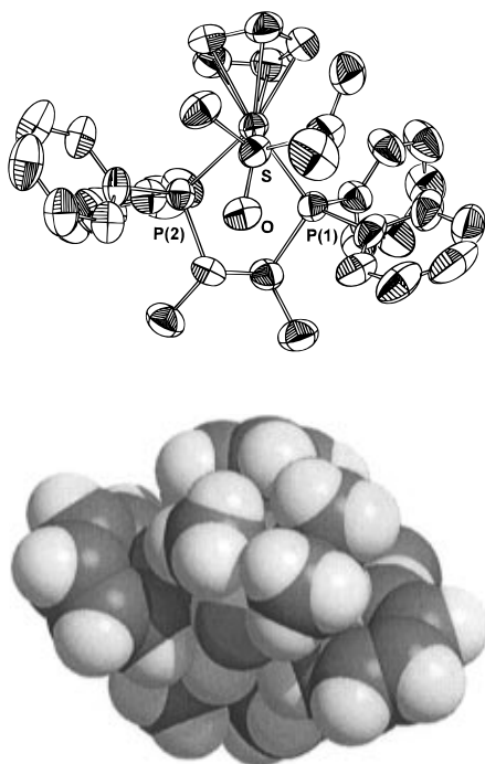
Figure 4. Ortep plot and space-filling model of the cation [\text{CpRu}(\text{chir})(\text{MeS}(\text{O})\text{-}i\text{-Pr})]^+ ( 10b + ).
