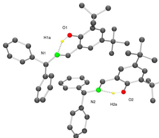
Figure 1. Representation of the asymmetric ur L 3 H (dpa). Hydrogen atoms attached to carbon been omitted for clarity. Dashed lines in intramolecular hydrogen bonds. Selected bond lengths (Å) and angles (°): O1–H1A 0.96(4), O1–N1 2.602(3), O2–H2A 1.02(4), O2...N2 2.597(3) Å; H1A...N1 149(4), O2–H2A...N2 154(3).
