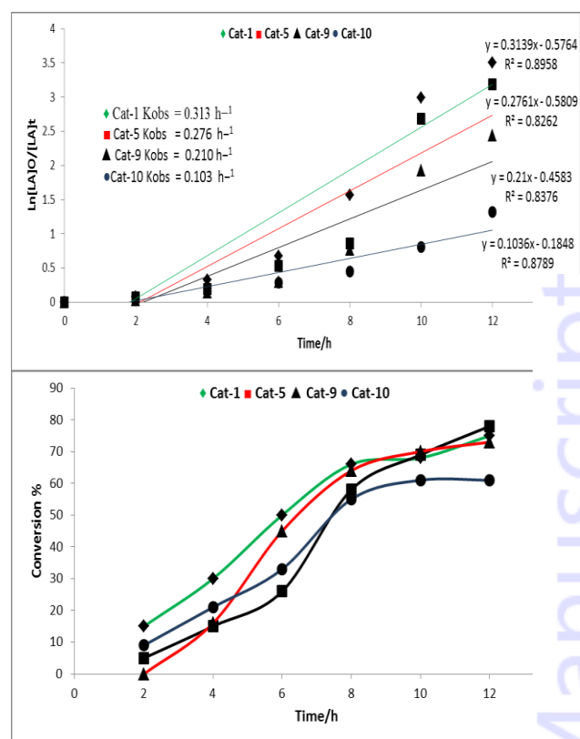
Figure 9. Top: Plot of \ln[\text{rac-LA}]_0/[\text{rac-LA}]_t vs time 1 , 5 , 9 and 10 ; Bottom: Relationship between conversion and time of polymerization rac -LA using 1 , 5 , 9 and
