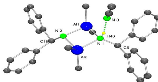
Figure 6. Molecular structure of [Ph 2 CHN(Me 2 Al)] 2 ·MeCN ( 11 ·MeCN), showing the numbering scheme. Most hydrogen atoms have omitted for clarity. Selected bond lengths (Å) angles (°): Al(1)–N(1) 1.9597(10), Al(1)–N(2) 1.9484(10), Al(2)–N(1) 1.9620(10), Al(2)–N(2) 1.9528(10), N(1)–C(5) 1.4771(14), N(2)–C(18) 1.4836(13); Al(1)–N(1)–Al(2) 91.72(4); Al(1)–N(1)–N(2) 92.35(4), N(1)–Al(1)–N(2) 86.67(4), N(1)–Al(2)–N(2) 87.48(4).
