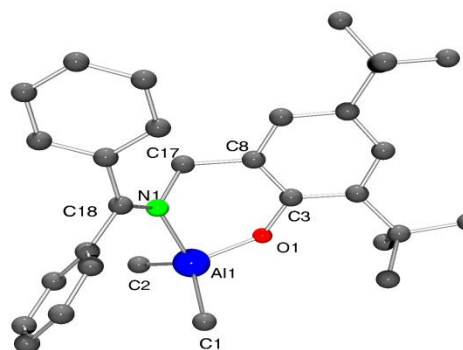
Figure 2. Molecular structure of [Ph 2 CHN=CH( t Bu 2 C 6 H 2 -O-2)AlMe 2 ] ( 5 ), showing the numbering scheme. Hydrogen atoms have omitted for clarity. Selected bond lengths (Å): Al(1)–O(1) 1.769(11), Al(1)–N(1) 1.991(14), Al(1)–C(1) 1.965(16), Al(1)–C(2) 2.001(16), N(1)–C(17) 1.317(19), N(1)–C(18) 1.522(19), C(17)–C(18) 1.50(2); O(1)–Al(1)–N(1) 92.5(6), C(1)–Al(1)–C(2) 118.0(10), Al(1)–O(1)–C(3) 125.7(11), Al(1)–N(1)–C(18) 126.0(9).
