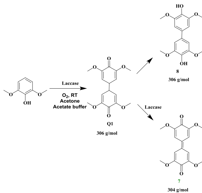
Scheme 3. Laccase-catalyzed dimerization of 2,6-dimethoxyphenol.
