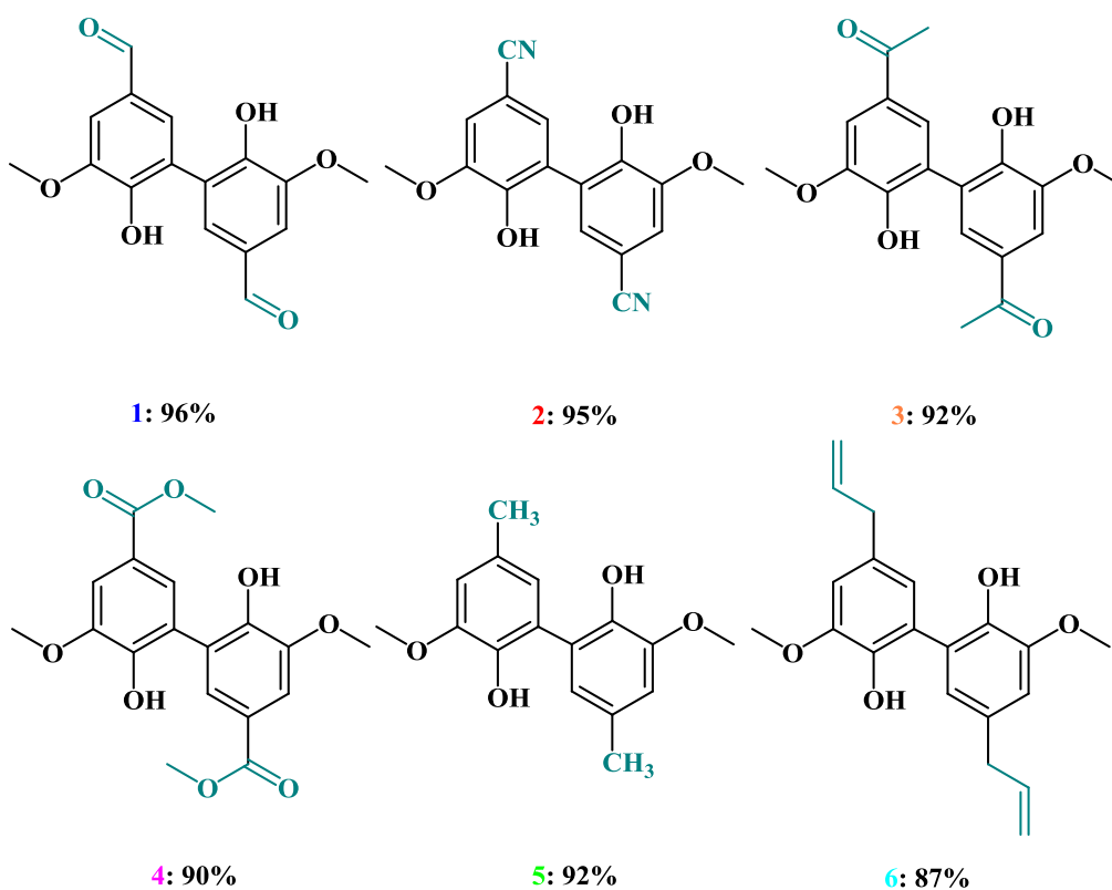
Scheme 2. Products of laccase-catalyzed selective dimerization of vanillin, 4-hydroxy-3-methoxybenzonitrile, acetovanillon, methylvanillate, 2-methoxy-4-methyl phenol and eugenol.
