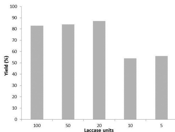
Figure 1. Divanillin yields depending on laccase quantity for 1.5 g of vanillin, in 200 mL of solvent, after 24 h.
