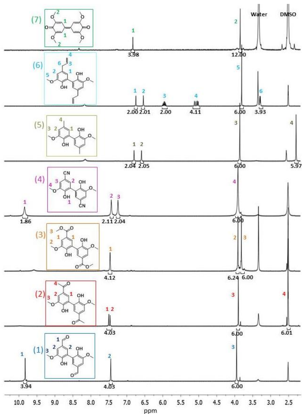
Figure 4. ^1\text{H} NMR spectra of the dimers obtained by selective oxidative coupling catalyzed by laccase of vanillin (1), acetovanillon (2), methylvanillate (3), 4-hydroxy-3-methoxybenzonitrile (4), 2-methoxy-4-methyl phenol (5), eugenol (6) and of 2,6-dimethoxyphenol (7).
