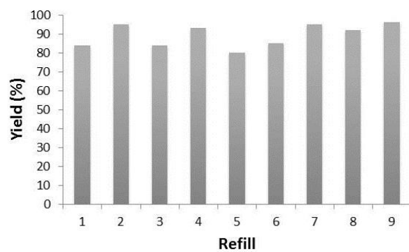
Figure 3. Divanillin yield, after 24 h of reaction under optimized conditions (20 U, acetate buffer) for the first reaction plus 8 refills.
