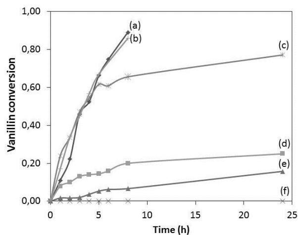
Figure 2. Vanillin conversion versus time using data extracted from ^1\text{H} NMR spectra (aldehyde signal): different conditions: (a) 10% acetone-90% acetate buffer/ \text{O}_2 , (b) 10% acetone-90% acetate buffer/air, (c) 10% acetone-90% water/ \text{O}_2 , (d) 40% acetone-60% acetate buffer/ \text{O}_2 , (e) 10% acetone-90% acetate buffer/ \text{N}_2 , (f) 70% acetone-30% acetate buffer/ \text{O}_2 .
