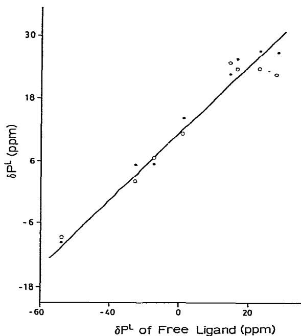
Fig. 3. A plot of the chemical shift of PL versus the chemical shift of the free ligand PL . * - point corresponding to the aminophosphine series. \circ - points corresponding to the S,S -chiraphos series.
