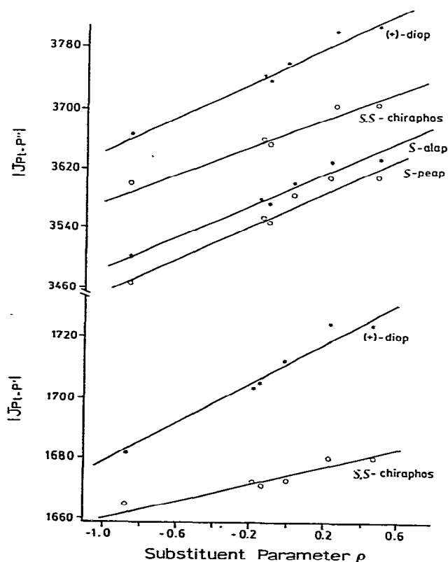
Fig. 4. Plot of the phosphorus—platinum coupling constants versus the Hammett substituent parameters of the para -substituted pyridines.
