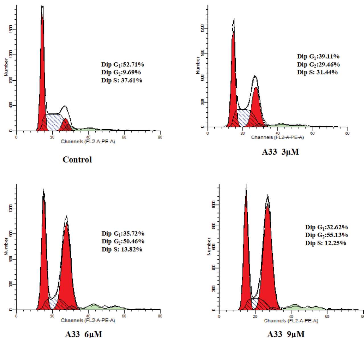
Figure 3. Cell cycle distribution induced by compound A33 was measured in MGC-803 cells. Cells were treated with compound A33 of 3, 6 and 9 \mu\text{M} for 48 h. Samples were analysed by flow cytometry and received results were analysed by modifit software.
