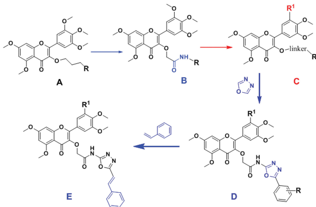
Figure 1. Design of the title compounds.
