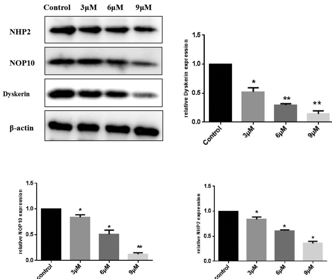
Figure 5. Compound A33 inhibited Dyskerin expression in MGC-803 cells. MGC-803 cells were treated with compound A33 of 3, 6 and 9 \mu M for 48 h. The proteins expression of Dyskerin, NOP10 and NHP2 were analysed by Western blotting. The results are expressed as relative expression against control expression. n = 3 . Results are shown as mean \pm SD from three independent experiments. * p < 0.05 , ** p < 0.01 .
