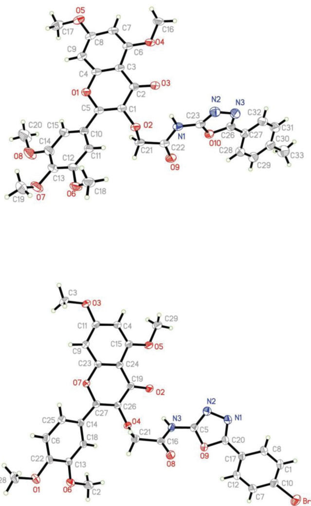
Figure 2. ORTEP drawing of compounds A11 and B8.
