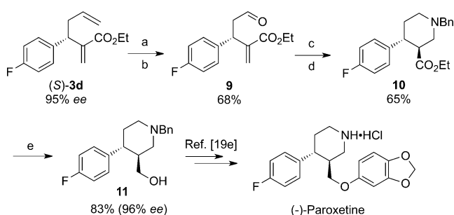
Scheme 3. Formal synthesis of (–)-Paroxetine. Reaction conditions: a) m CPBA (1.5 equiv), CH 2 Cl 2 , 0 °C–RT, 17 h; b) HIO 3 (1.2 equiv), THF/H 2 O (3:1), 0 °C, 1 h; c) BnNH 2 (3 equiv), NaBH 3 CN (5 equiv), AcOH (6 equiv), MeOH, RT, 17 h; d) t BuOK (3 equiv), t BuOH (1.5 equiv), toluene, RT, 1 h; e) LiAlH 4 (10 equiv), THF, 0 °C, 1 h. m CPBA = m -chloroperbenzoic acid.
