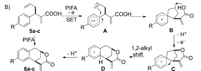
Scheme 2. A) Synthetic utility of the cross-coupling products in the preparation of the polycyclic lactones 6a-c and polycyclic lactams 8a-c . Reaction conditions: a) 3a-c , LiOH, THF/H 2 O (1:1), reflux, 24 h; b) 5a-c , PIFA, Sc(OTf) 3 , CH 3 CN, 0 °C, 12 h; c) 5a-c , p -toluenesulfonyl isocyanate (PTSI), Et 3 N, THF, 60 °C, 3 h; d) 7a-c , PIFA, Sc(OTf) 3 , CH 3 CN, 0 °C, 12 h. X-ray structure of 6a is shown with thermal ellipsoids at 50% probability. [20] B) Proposed mechanism for PIFA-mediated oxidative cyclizations of 5 . PIFA = phenyliodine bis(trifluoroacetate), THF = tetrahydrofuran, Ts = 4-toluenesulfonyl.
