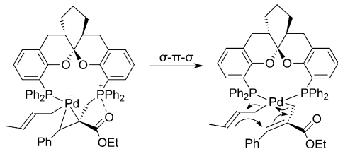
Scheme 1. Proposed model for inner-sphere 3,3'-reductive elimination in allyl-allyl cross-coupling.
