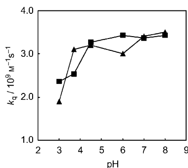
Figure 3. pH-dependent variation of the fluorescence quenching rate constant ( k_q ) for AcrH + (■) or DCA (▲) photosensitizing one-electron oxidation of d m C in anoxic phosphate buffer solution (5 mM; pH 3.0–8.0).
