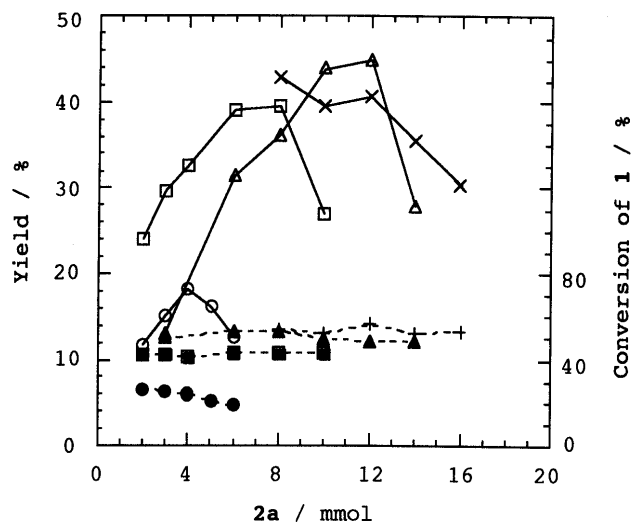
Fig. 1. Yields of 3-Ethoxymethylplumbagin ( 3a ) and Conversion of Plumbagin ( 1 ) in the Reaction of 1 (1 mmol) with Ethoxyacetic Acid ( 2a ) in the Presence of Various Amounts of \text{Pb}(\text{OAc})_4
