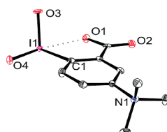
Figure 2. Perspective drawing of 1a with 50% ellipsoid probability. selected bond distances [Å]: I(1)–O(4) 1.8012(19), I(1)–O(3) 1.8150(19), I(1)–O(1) 2.498.
