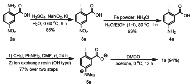
Scheme 1. Synthetic Route of AIBX 1a
