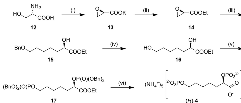
FIGURE 6. Synthesis of enantiopure inhibitor 4. Yields are given for the synthesis of (R)-4; analogous procedures using L-serine as the starting material were used for the synthesis of (S)-4 in comparable yields. Please refer to the supplemental material for more detail. (i) \text{HNO}_2 , KBr, \text{H}_2\text{O} then KOH/EtOH, 37% (two steps). (ii) EtBr, \text{Bn}(\text{Et})_3\text{NCl} , \text{CH}_2\text{Cl}_2 , 66%. (iii) \text{BnO}(\text{CH}_2)_4\text{Br} , magnesium, tetrahydrofuran, room temperature, then \text{CuBr}\cdot\text{SMe}_2 , -78^\circ\text{C} , then 14, 32%. (iv) \text{H}_2 , palladium/carbon, EtOAc, 66%. (v) (\text{BnO})_2\text{P}-\text{N}(\text{Pr})_2 , 1 H -tetrazole, dichloromethane, then meta -chloroperbenzoic acid 64%. (vi) \text{H}_2 , palladium/carbon, EtOAc, then KOH/ \text{H}_2\text{O} , then DOWEX- \text{H}^+ , anion exchange chromatography, 27%.
