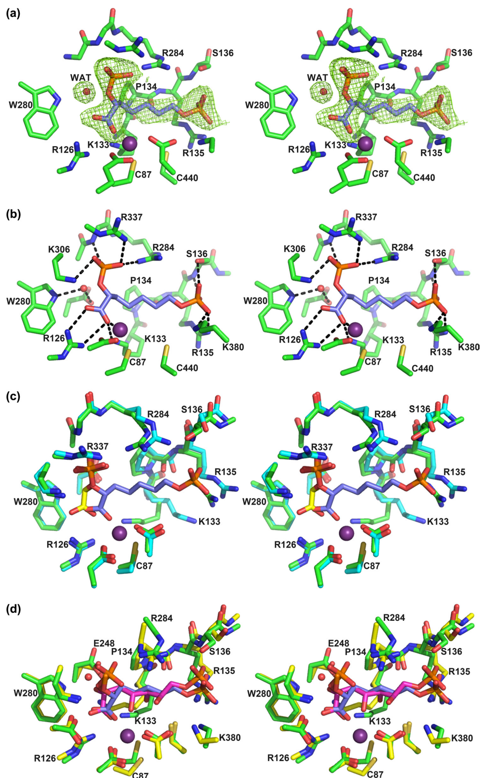
FIGURE 5. Stereo view of the active site of the enzyme in complex with inhibitor 4 (only the (R)-enantiomer is shown for clarity). a , |F_o - F_c| simulated annealing omit map contoured at 3\sigma showing the electron density for inhibitor 4 (blue carbons) in the active site. WAT, water. b , interactions of 4 with the active site residues (green carbons) and metal ion (purple sphere). c , overlay of P-enolpyruvate (yellow carbons)-DAH7PS structure 3NV8 (cyan carbons) with DAH7PS-4-complex (green carbons). d , overlay of the preferred pose of the linear intermediate (magenta carbons) and 4 (blue carbons; the oxygens on the C2-phosphate were omitted for clarity). The enzyme structure experimentally obtained from the DAH7PS-4-complex (green carbons) superimposes well onto the enzyme structure obtained by induced fit modeling of the linear intermediate (yellow carbons, peptide; magenta carbons, intermediate).
