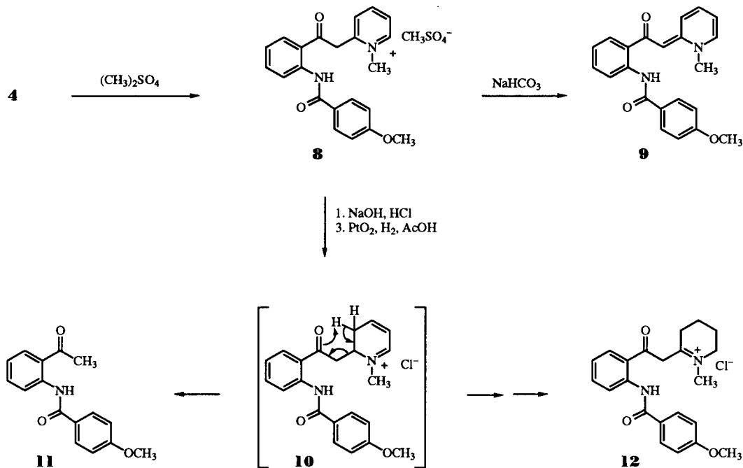
Scheme IV
