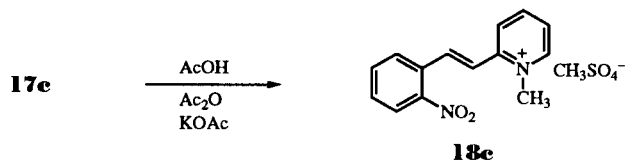
Scheme IX
