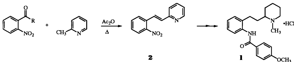
Scheme II
