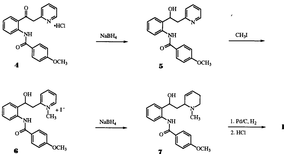
Scheme III
