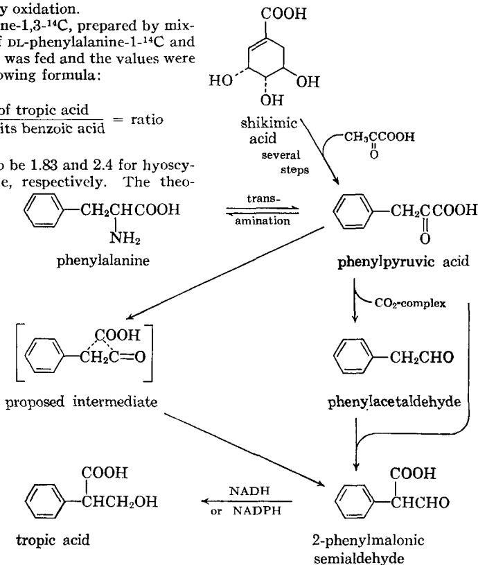
Proposed Biosynthetic Pathway for Tropic Acid
