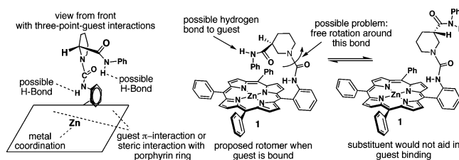
Scheme 2. Possible Binding Interactions of Host 1 with Guests and Proposed Host Conformations
