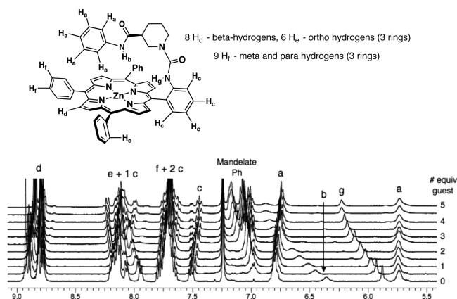
Figure 5. ^1\text{H} NMR titration of host 1 with ( R )-mandelate (0.5 equiv additions).
