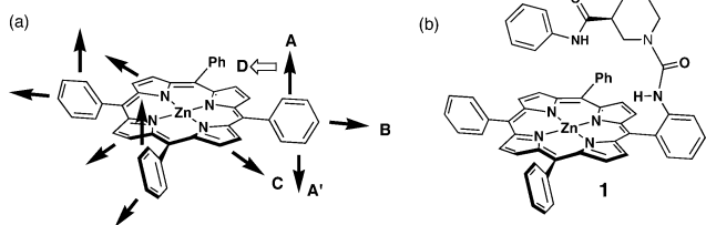
Figure 1. (a) Porphyrin design strategies. (b) Receptor 1 .
