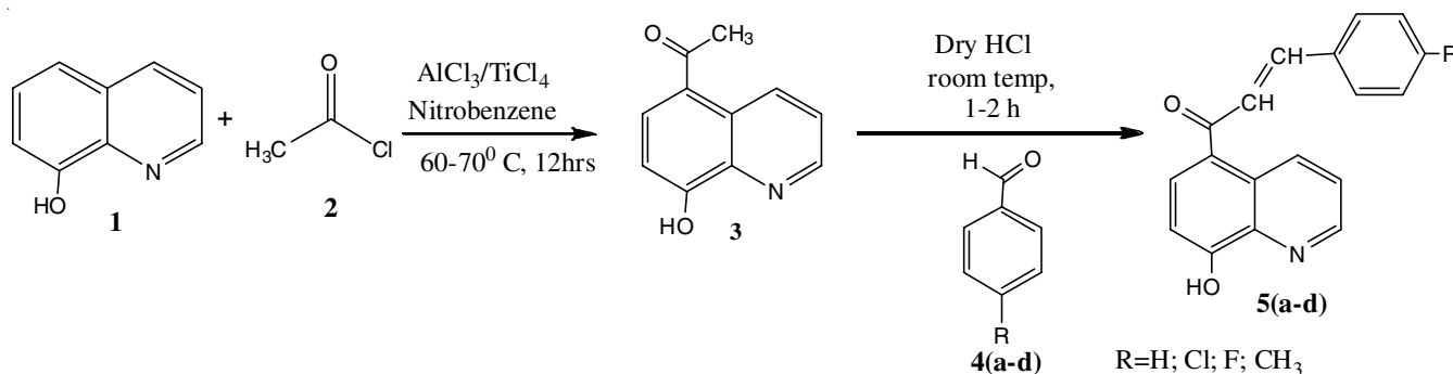
Scheme-I: Reaction pathway for the synthesis of 1-(8-hydroxyquinolin-5-yl)-3-(aryl)prop-2-en-1-one 5(a-d)
