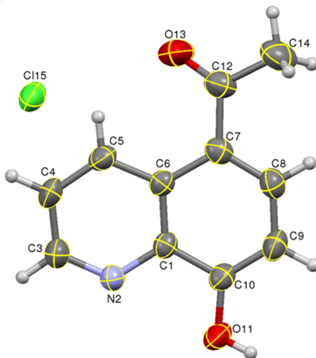
Fig. 1. ORTEP of the molecule 5-acetyl-8-hydroxyquinoline ( 3 ) drawn at 50% probability level
