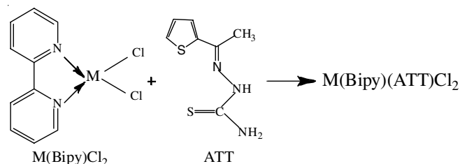
Scheme-I: Synthesis of mixed ligand metal complexes [where, M = Cu(II), Ni(II), Co(II)]
