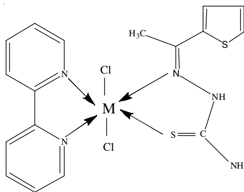
Fig. 5. Structure of M(Bipy)(ATT)Cl 2 complex
