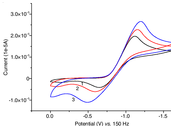
Fig. 6. Cyclic voltammogram of Ni(Bipy)(ATT)Cl 2 · 0.5 H 2 O, at different scan rates (1) 0.05 (2) 0.1 (3) 0.2 mV s -1
