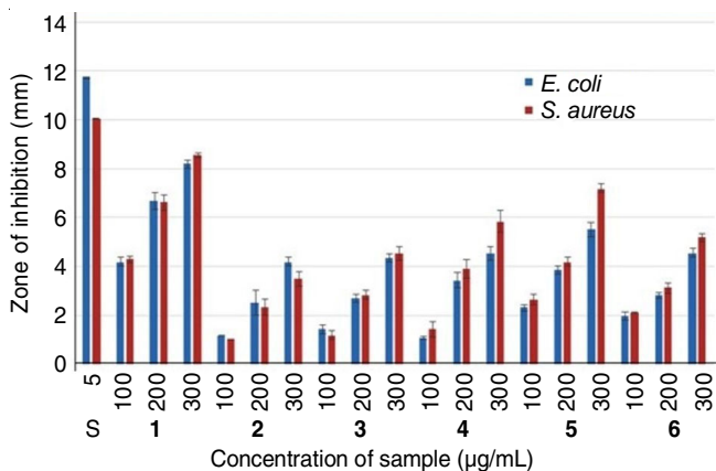
Fig. 8. Graphical representation of antibacterial activity of metal complexes against pathogenic bacterial strains
