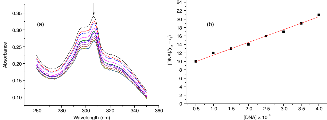
Fig. 7. Absorption spectra of Ni(Bipy)(ATT)Cl 2 ·0.5H 2 O. In the absence and in the presence of increasing concentration of CT-DNA; [(a) most spectrum is recorded in the absence of CT-DNA and (b) spectra on addition 20 \mu\text{L} DNA each time] A plot [\text{DNA}]/(\epsilon_a - \epsilon_f) vs. [\text{DNA}] \times 10^6 is shown
