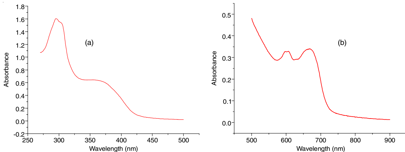
Fig. 3. Electronic spectrum of Co(Bipy)(ATT)Cl 2 complex (a) in lower concentration and (b) in higher concentration
