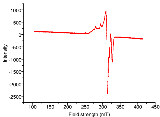
Fig. 4. ESR spectrum of Cu(Bipy)(ATT)Cl 2 complex (LNT)
