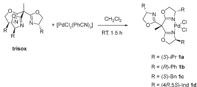
Scheme 1. Synthesis of palladium(II) complexes 1a–1d .
