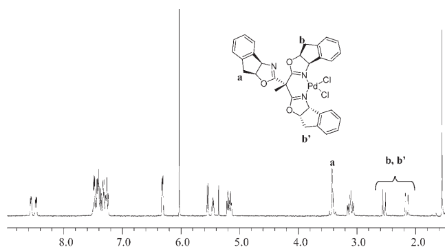
Figure 10. 1 H NMR of complex [PdCl 2 (Ind-trisox)] ( 1d ) in 1,1,2,2-[D 2 ]tetrachloroethane at 296 K (400 MHz).
