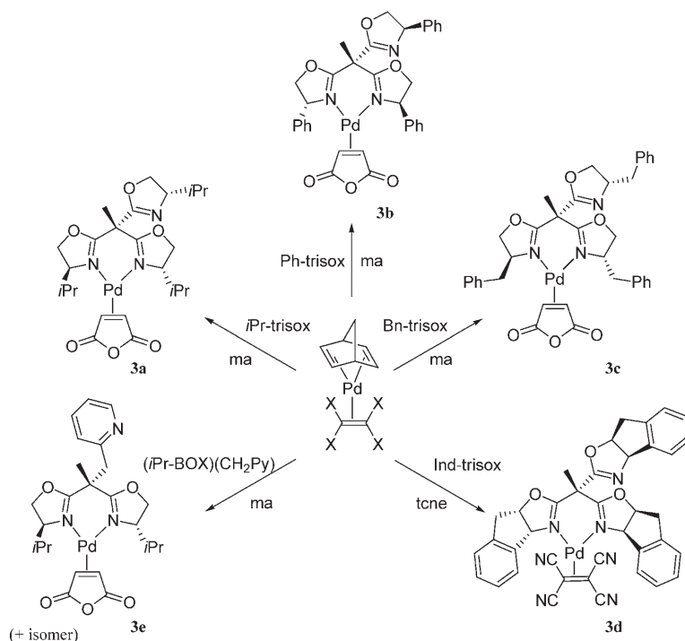
Scheme 4. Palladium(0) complexes 3a–e (nbd = norbornadiene, ma = maleic anhydride, tcne = tetracyanoethylene).
