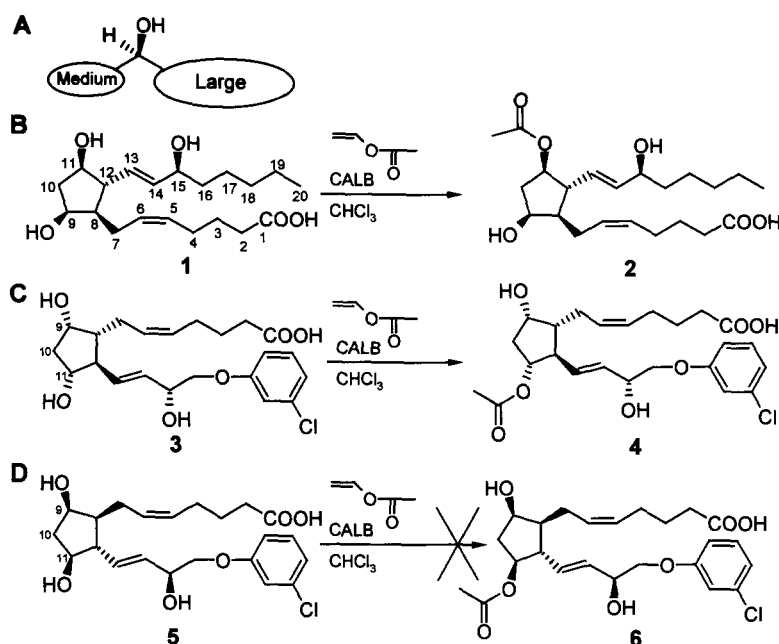
Figure 1. The enantio- and regioselective acetylation of prostanoids of F type catalysed by CALB.
