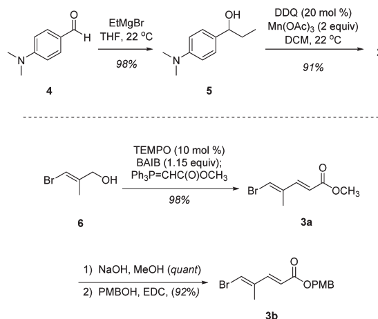
Scheme 2. Synthesis of Ketone 2 and Alkenyl Bromides 3a and 3b
