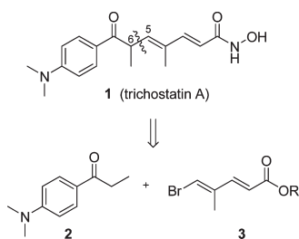
Scheme 1. Retrosynthetic Analysis of (±)-TSA (1)
