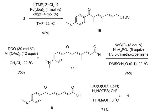
Scheme 4. Synthesis of (±)-TSA Using Alkenyl Bromide 9
