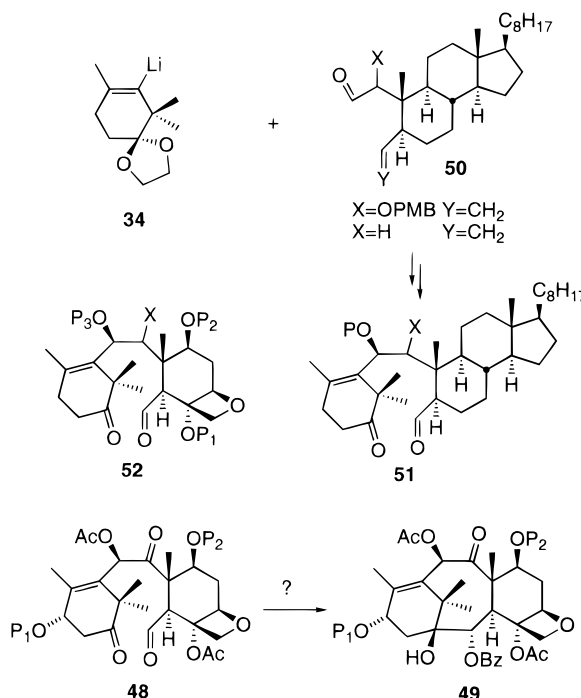
Scheme 16
