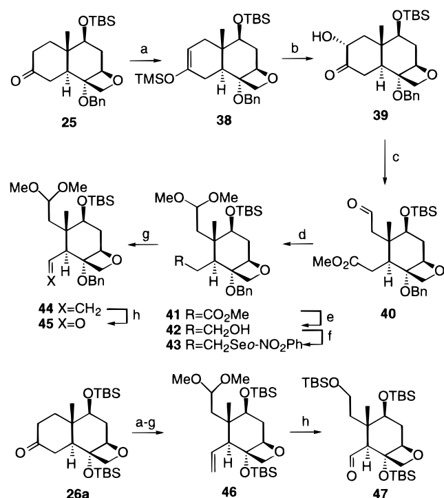
Scheme 14 a
