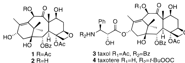
Figure 1. Structures of baccatin III ( 1 ), 10-deacetylbaccatin III ( 2 ), taxol ( 3 ), and taxotere ( 4 ).
