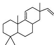
2: generic structure of pimarane diterpenes
