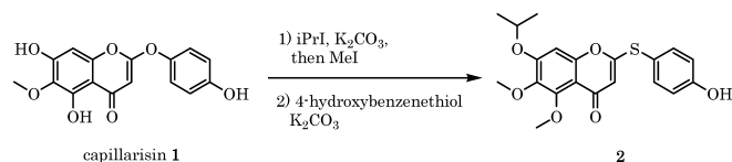
Chart 1. Conversion of Capillarisin 1 to Sulfur-Analogue 2
