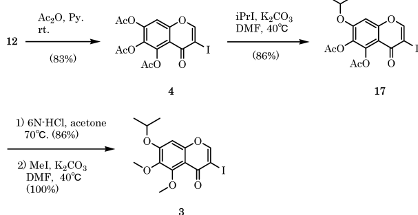
Chart 4. Synthesis of Key Intermediate 3 via 4
