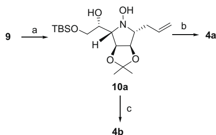
Scheme 2. Reagents and conditions: (a) allylmagnesium chloride, THF, 0–25 °C, 75%; (b) TFA–H 2 O, 9:1 ratio, 0–25 °C, 6 h, 80%; (c) (i) Zn, MeOH–acetic acid 20:1 ratio, reflux 3 h, (ii) TFA–H 2 O, 9:1 ratio, 0–25 °C, 6 h, 82%.
