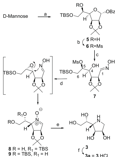
Scheme 1. Reagents and conditions: (a) Ref. 10; (b) MsCl, Et 3 N, DCM, 3 h, 98%; (c) (i) K 2 CO 3 , MeOH, 25 °C, 0.5 h, 98%; (ii) hydroxylamine hydrochloride, NaHCO 3 , MeOH–H 2 O, rt for 3 h, 90%; (d) hydroxylamine hydrochloride, NaHCO 3 , MeOH–H 2 O, reflux for 12 h, 80% in the 2:8 ratio; (e) (i) H 2 , Pd/C, 12 h, (ii) TFA, H 2 O, (9:1), 0–25 °C, 6 h, 75%; (f) MeOH, HCl, 25 °C, 2 h, 98%.
