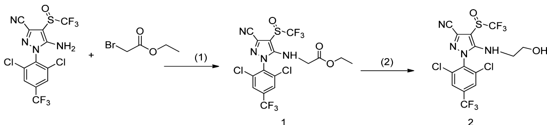
Scheme 1. Reagents and Conditions: (1) \text{NaH} , THF, and 2 h and (2) \text{NaBH}_4 , \text{ZnCl}_2 , THF, 50 ^\circ\text{C} , and 1 h
