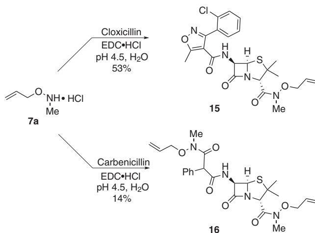
Scheme 7 Coupling of 7a to penams.
