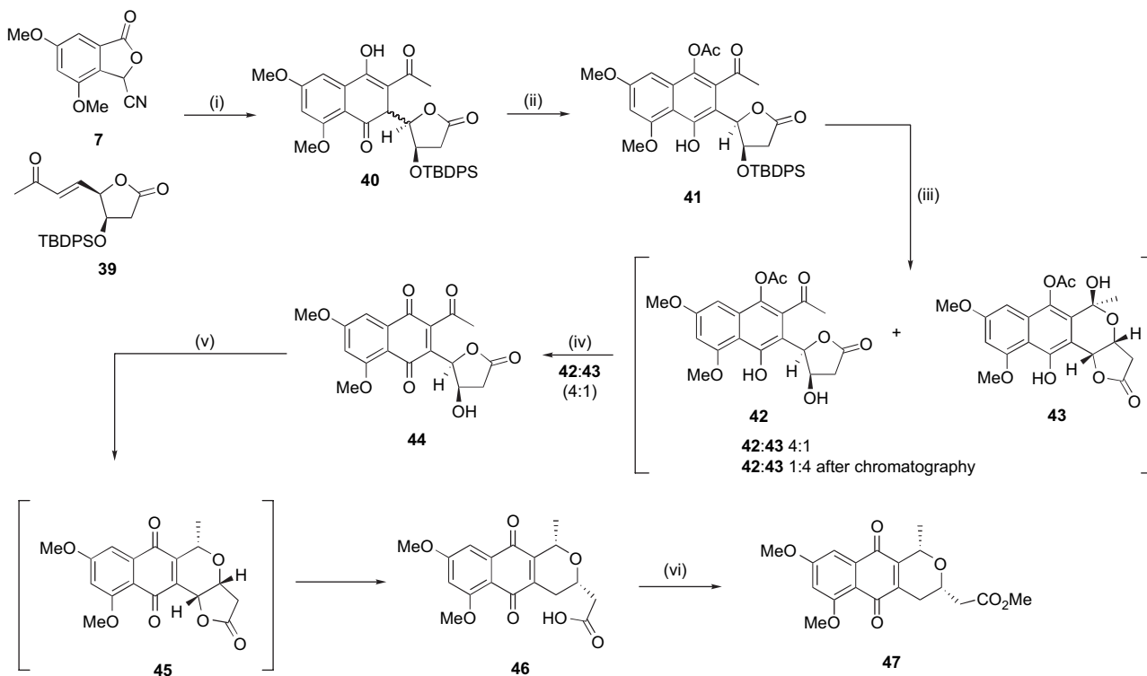
Scheme 13. (i) KO t Bu, DMSO, rt, 80%; (ii) BF 3 ·Et 2 O, CH 2 Cl 2 , –78 °C to 0 °C then Ac 2 O, py, –10 °C to rt, 53% over two steps; (iii) HF·Py, THF, rt, then SiO 2 (42/43=4:1); (iv) CAN, MeCN–H 2 O (2:1), 38% from 41; (v) BF 3 ·Et 2 O (10 equiv), Et 3 SiH (10 equiv), CH 2 Cl 2 , –78 °C to rt, 63%; (vi) MeOH, O 2 , dark, 32%.
