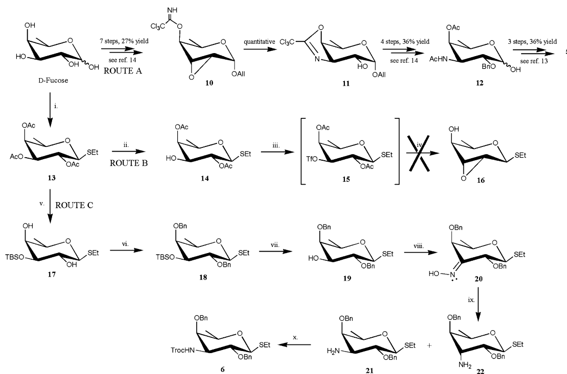
Scheme 2. Synthesis of D-Fucp3NAc donors 5 13 and 6 . Reagents and conditions: i: (a) \text{Ac}_2\text{O} , py, rt, (b) \text{I}_2 , \text{Et}_3\text{SiH} , \text{CH}_2\text{Cl}_2 , reflux, (c) thiourea, \text{CH}_3\text{CN} , 60\text{ }^{\circ}\text{C} then EtI, \text{Et}_3\text{N} , rt, 74% over three steps; ii: (a) t\text{-BuOK} , MeOH, 0\text{ }^{\circ}\text{C} , (b) CSA, 7:2 v/v \text{MeC(OMe)}_3/\text{DMF} , 100 mbar, rt, (c) \text{Ac}_2\text{O} , py, rt, (d) 80% \text{AcOH} , rt, 82% over four steps; iii: \text{TF}_2\text{O} , 1:1 v/v py/ \text{CH}_2\text{Cl}_2 , 0\text{ }^{\circ}\text{C} ; iv: Na, 1:1 v/v MeOH/ \text{CH}_2\text{Cl}_2 , 0\text{ }^{\circ}\text{C} ; v: (a) t\text{-BuOK} , MeOH, 0\text{ }^{\circ}\text{C} , (b) TBSCl, ImH, DMF, 0\text{ }^{\circ}\text{C} , 79% over two steps; vi: BnBr, NaH, DMF, 0\text{ }^{\circ}\text{C} , 93%; vii: TBAF, THF, rt, 98%; viii: (a) 2:1 v/v DMSO/ \text{Ac}_2\text{O} , rt, (b) \text{NH}_2\text{OH}\cdot\text{HCl} , NaOAc, MeOH, rt, 78% over two steps; ix: Red-Al ® , THF, 0\text{ }^{\circ}\text{C} , 21 : 80%, 22 : 8%; x: TrocCl, py, 82%.
