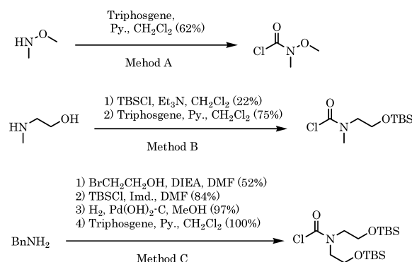
Chart 1. Typical Synthetic Methods for Carbamoyl Chlorides (Method A, B and C)
