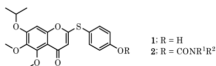
Fig. 1. Parent Compound 1 and its Prodrugs 2
