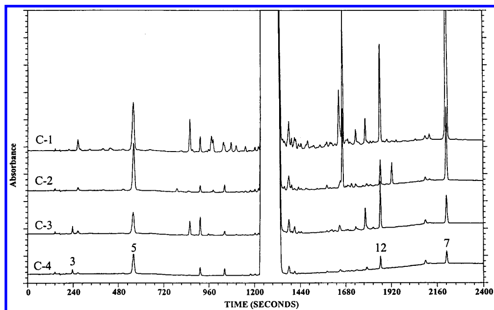
Figure 6. Gradient HPLC chromatograms of 1 produced by Route C, C-1; from crude 3 , C-2; from crystallized 3 , C-3; recrystallization of 1 from sample C-1, C-4; recrystallization of 1 from sample C-2.
