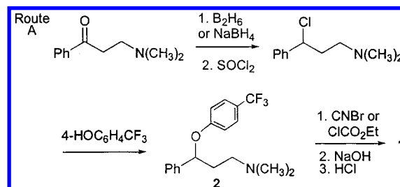
Figure 1. Original reported synthesis of 1 , Route A.
