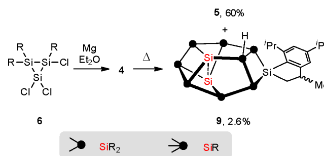
Scheme 2. Isolation of 9 as a Side Product in the Synthesis of the Global Minimum Isomer 5 a
