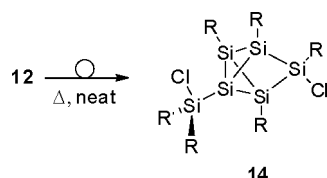
Scheme 5. Thermal Rearrangement of 12 to 14 a
