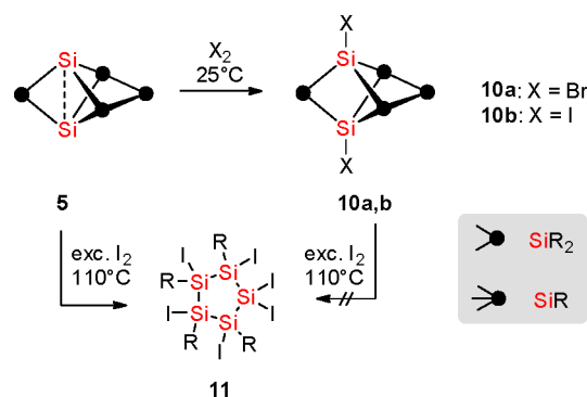
Scheme 3. Halogenation of Siliconoid 5 to 1,5-Dihalo Derivatives 10a,b 15 and Contraction to Hexaiodocyclopentasilane 11 a
