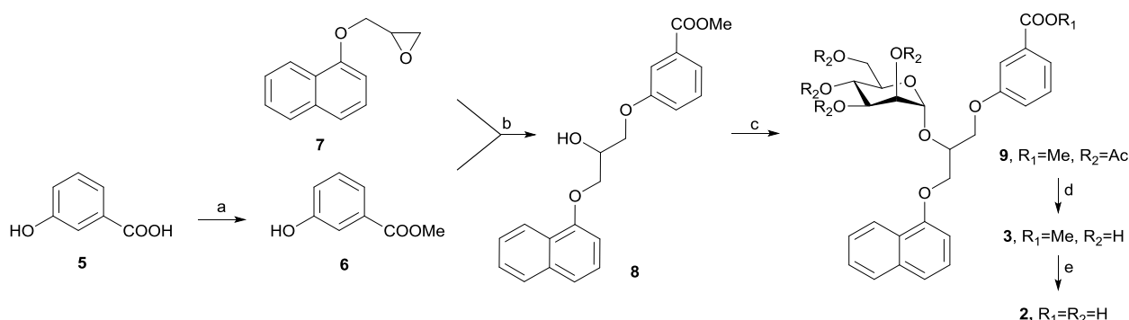
Scheme 1 Reagents and conditions: a) SOCl 2 , MeOH, r.t., 24 h; b) (i) KOH, MeOH, r.t., 20 min; (ii) tetrabutylammonium bromide, toluene/ N,N -dimethylformamide, 90 °C, 20 h; c) 2,3,4,6-tetra- O -acetyl- \alpha -D-mannopyranosyl trichloroacetimidate, TMSOTf, CH 2 Cl 2 , 0 °C, then r.t., 24 h; d) NaOMe, MeOH, 1 h, then Amberlite® IR120 H, 10 min; e) 1 M NaOH, EtOH, r.t., 24 h.
