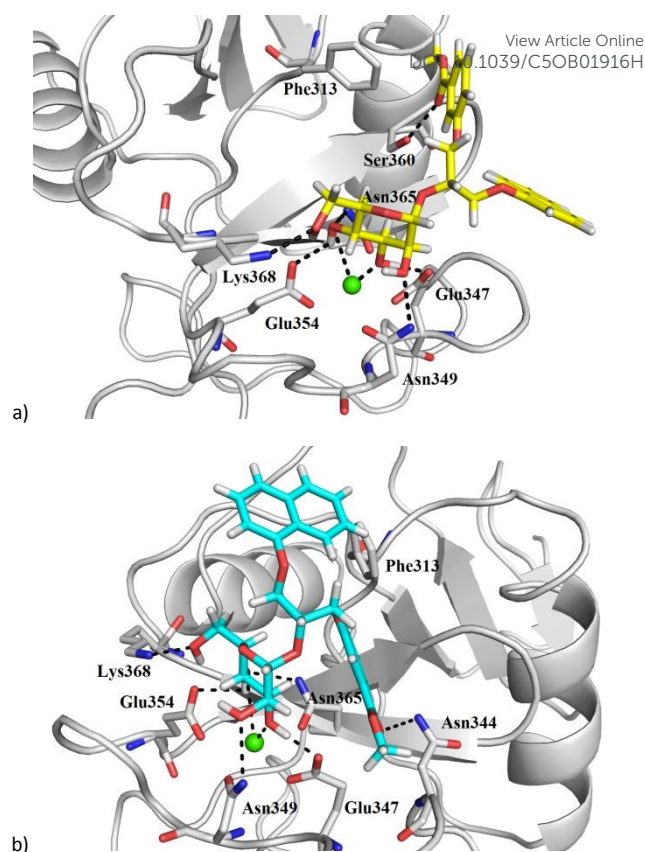
Fig. 7. FlexX docking poses of compounds a) ( R )- 3 (in yellow sticks) and b) ( S )- 3 (in cyan sticks) in DC-SIGN CRD Ca 2+ -binding site. Protein (PDB entry: 1SL4) is presented in grey cartoon and Ca 2+ ion as a green sphere. For clarity only side chains of amino acid residues predicted to interact with the docked ligands are shown as grey sticks. Hydrogen bonds are shown as black dashed lines. Figure was prepared by PyMOL. 26
