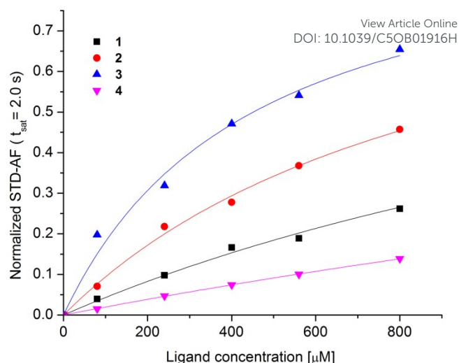
Fig. 6 Normalized STD-AF curves as a function of ligand concentration in the range from 80 to 800 \mu\text{M} . Experimental data were collected at 25 ^{\circ}\text{C} , 2.0 s saturation time on a 600 MHz NMR spectrometer with 8 \mu\text{M} DC-SIGN concentration in 25 mM Tris- \text{d}_{11} (pD = 8.0), 150 mM NaCl, 4 mM \text{CaCl}_2 and 25% DMSO- \text{d}_6 in ^2\text{H}_2\text{O} . Experimental data were fitted to the Eq. 3 (1: K_D = 1.6 \pm 0.5 mM, R^2 = 0.992 , 2: K_D = 0.96 \pm 0.08 mM, R^2 = 0.999 , 3: K_D = 0.45 \pm 0.05 mM, R^2 = 0.997 , 4: K_D = 4.9 \pm 0.7 mM, R^2 = 0.999 ).
