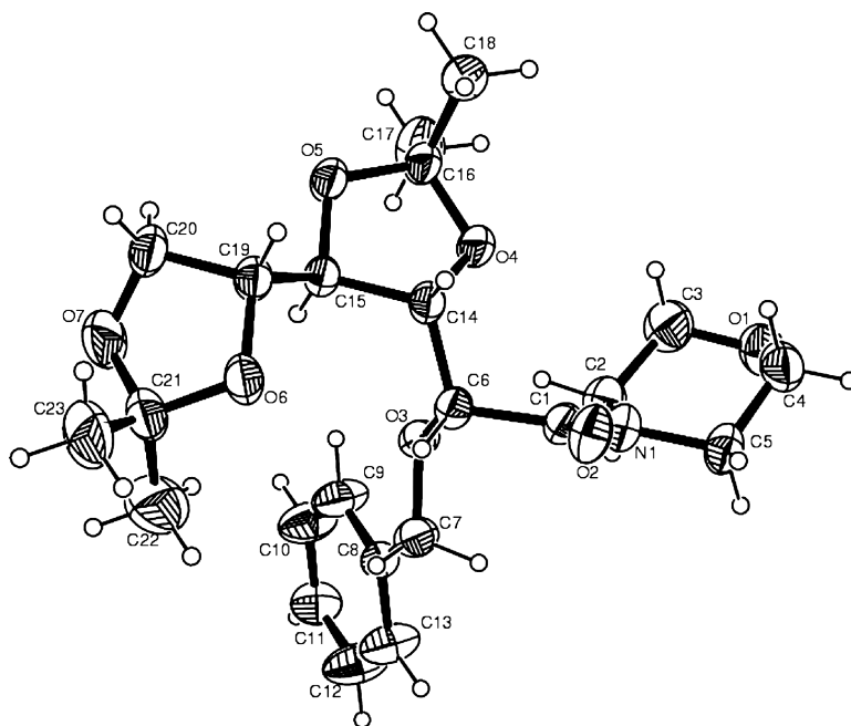
Figure 2. ORTEP plot (8) of compound 9a with thermal ellipsoids drawn at 50% probability level (Johnson, 1976).
