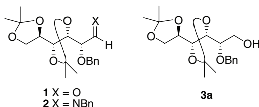
Figure 1: 2- O -benzyl glucitol derivative 3a —A precursor of valuable intermediates 1 and 2 .
