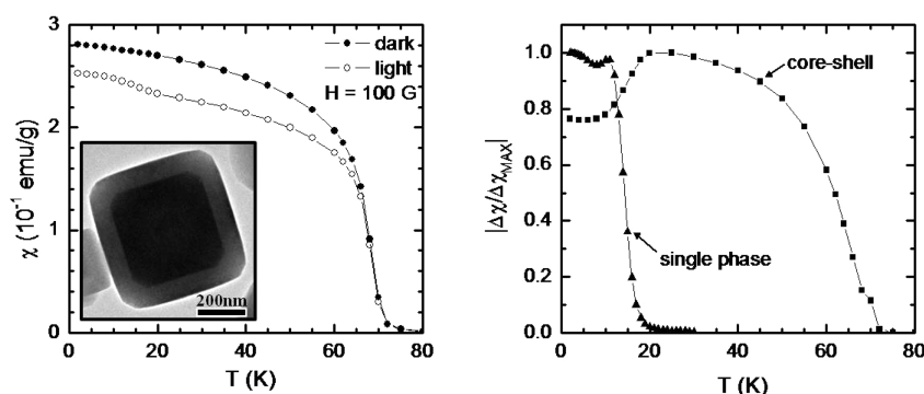
Figure 4. (a) Field-cooled magnetic susceptibility, \chi , of BA as a function of the temperature before irradiation (●, “dark”) and with the light off after 11 h of irradiation with visible white light (○, “light”). Lines are guides for the eyes. The inset is a HRTEM picture of a RbCoFe/KNiCr heterostructure. (b) Magnitude of the photoinduced change in \chi , \Delta\chi = \chi(\text{light}) - \chi(\text{dark}) , normalized to the maximum value: (■) data for the core/shell particles from the left panel; (▲) data for a single-phase Co/Fe PBA powder taken from ref 30. Lines are guides for the eyes.
