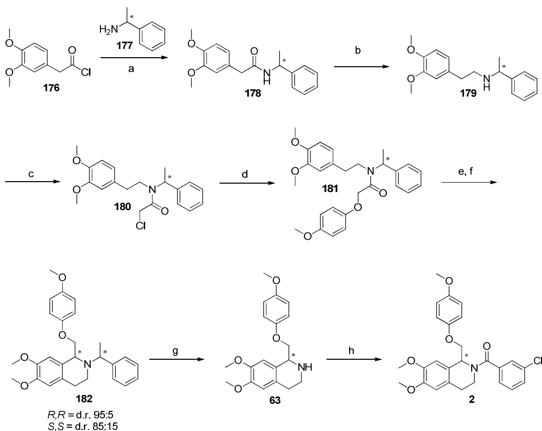
Scheme 7. a) NaOH, DCM/H 2 O, R = 72%, S = 82%; b) BF 3 ·OEt 2 O, then BH 3 ·THF, THF, R = 90%, S = 95% c) 2-chloroacetyl chloride, Et 3 N, DCM, R = 80%, S = 73%; d) 4-methoxyphenol, Cs 2 CO 3 , MeCN, R = 74%, S = 73%; e) POCl 3 , toluene, reflux; f) NaBH 4 , MeOH, -78 °C, R , R = 34%, S , S = 34%; g) H 2 , Pd/C, EtOH; h) 3-chlorobenzoyl chloride, Et 3 N, DCM, R = 51%, S = 34%.
