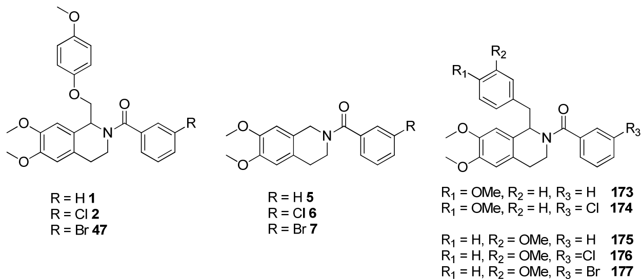
Figure 4. Structure of analogues with B-ring and linker B removed (5-7) and analogues with a one atom linker B (173-177)
