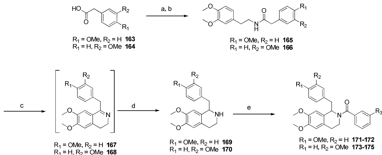
Scheme 6. a) SOCl 2 , DCM; b) 3,4-dimethoxyphenethylamine, Et 3 N, DCM, 26-84% over two steps; c) POCl 3 , toluene, reflux ( Procedure IV ); d) NaBH 4 , MeOH, 18h, 26% over two steps ( Procedure VI ); e) substituted benzoyl chloride, Et 3 N, DCM, 31-64% ( Procedure VII ).
