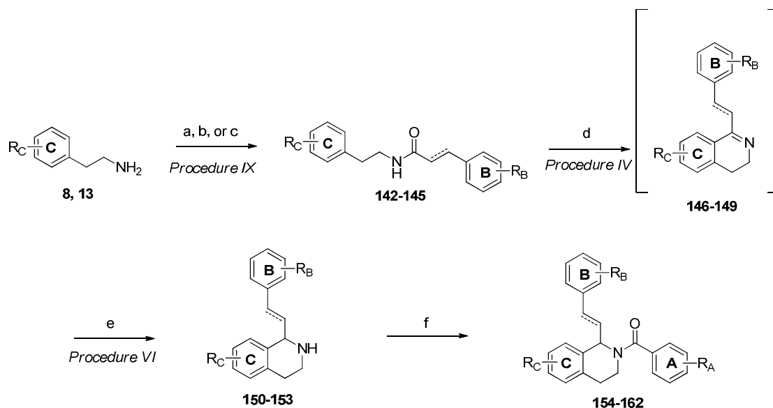
Scheme 5. a) 4-methoxycinnamic acid, EDC, DMAP, DMF/DCM, 18h, 42-66% ( Procedure IX ); b) 4-methoxyphenylpropionic acid, EDC, DMAP, DCM/DMF, 18h, 66% ( Procedure IX ); c) phenylpropionyl chloride, Et 3 N, DCM, 99%; d) POCl 3 , toluene, reflux, 1.5h ( Procedure VI ); e) NaBH 4 , MeOH, 18h, 58-73% over two steps ( Procedure VI ); f) substituted benzoyl chloride, Et 3 N, DCM, 0°C, 38-84% ( Procedure VII ).
