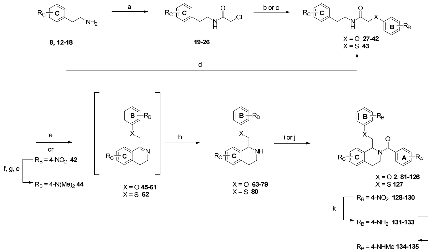
Scheme 3. a) chloroacetyl chloride, Et 3 N, DCM, 0°C, 1.5-2h, 68-83% ( Procedure II ); b) substituted phenol, Cs 2 CO 3 , MeCN, 18h, 66-90% ( Procedure III ); c) 4-nitrophenol, CsF, DMF, 76%; d) phenoxyacetyl chloride, Et 3 N, DCM, 0°C, 1.5-2h, 69%; e) POCl 3 , toluene, reflux, 1.5-12 hrs ( Procedure IV ); f) Pd/C, H 2 , MeOH, 97%; g) paraformaldehyde, NaCNBH 3 , MeOH, 89%; h) NaBH 4 , MeOH, 18h, 18-70% over two steps ( Procedure VI ); i) substituted benzoyl chloride, Et 3 N, DCM, 0°C, 2h, 21-99% ( Procedure VII ); j) substituted benzoic acid, EDCI, DMAP, 18h, 22-68% ( Procedure VIII ); k) tin(II)chloride dihydrate, EtOH 33-66%; l) NaOMe, paraformaldehyde, sodium borohydride, MeOH, 68-72%.
