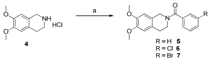
Scheme 1. a) substituted benzoyl chloride, \text{NaHCO}_3 , \text{DCM}/\text{H}_2\text{O} , 67-85% ( Procedure I ).
