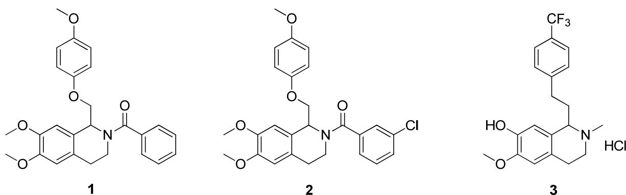
Figure 1. Structures for (6,7-dimethoxy-1-((4-methoxyphenoxy)methyl)-3,4-dihydroisoquinolin-2(1H)-yl)(phenyl)methanone (1), CIQ (2) and HON0001 (3).
