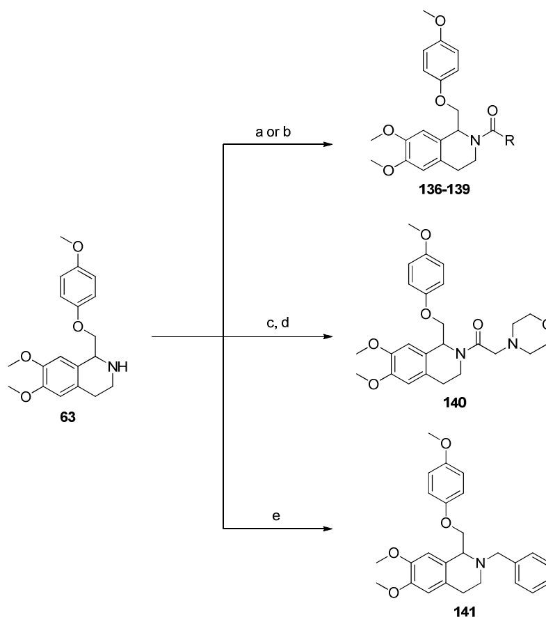
Scheme 4. a) aryl chloride, Et 3 N, DCM, 0°C, 21-99% ( Procedure VII ); b) 4-morpholinecarbonyl chloride, Et 3 N, DCM, 0°C, 31%; c) chloroacetyl chloride, Et 3 N, DCM, 0°C, 78%; d) morpholine, EtOH, 53%; e) BnBr, K 2 CO 3 , DMF, 39%.
