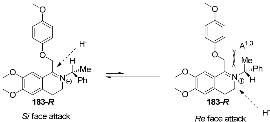
Figure 3. Proposed model to predict stereochemical outcome of the reduction of iminium 185-R
