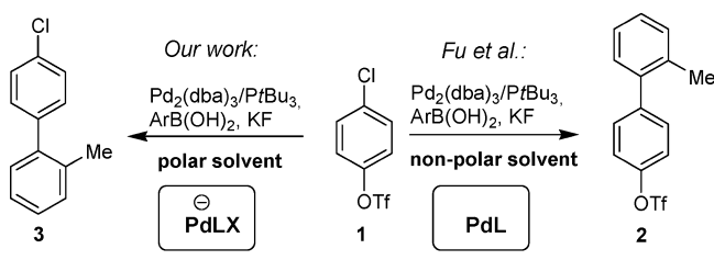
Additive effect in polar solvent on selectivity in Stille coupling:
