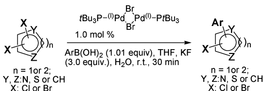
Scheme 1. Selective Couplings of Dihalogenated Heterocycles
