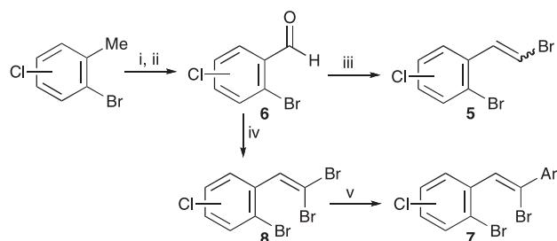
Scheme 2. The preparation of the tri- and tetrahalogenated starting materials. Reagents: (i) NBS, AIBN, CCl 4 ; (ii) NMO, MeCN; (iii) [Ph 3 PCH 2 Br] 2 , t BuOK; (iv) CBr 4 , PPh 3 , CH 2 Cl 2 ; (v) Pd 2 (dba) 3 , P(2-furyl) 3 , Na 2 CO 3 , Ar-B(OH) 2 .
