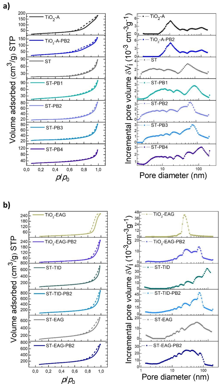
Figure 7. N 2 adsorption-desorption isotherms and pore size distribution (PSD) of (a) ST, ST-PB samples with different PB loadings, TiO 2 and TiO 2 -PB particles and (b) different silica-titania and titania aerogels before and after modification with similar amounts of PB.
