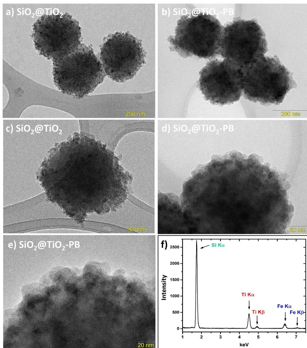
Figure 6. TEM images of (a,c) pristine ST core-shell particles in low (a) and higher (c) magnification, and (b,d,e) PB-modified sample (ST-PB3) in low (b) and higher magnification (d,e); (f) The EDS spectrum of the same ST-PB3 sample.
