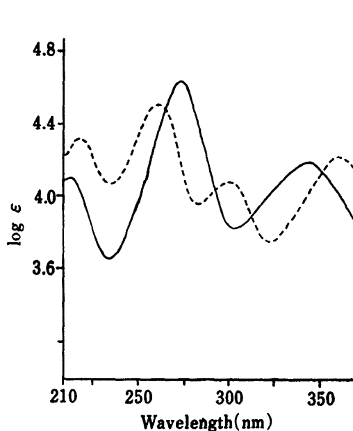
Fig. 1. UV Spectra of Compounds 5b (—) and 12 (---) in EtOH
