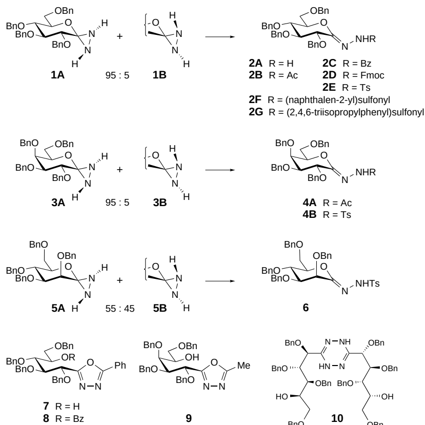
Scheme 2
