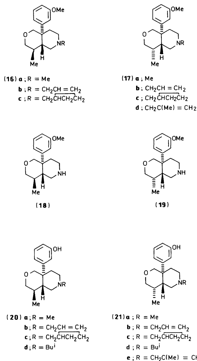
Scheme 2. Reagents: i, (a) BuLi, THF, -20^{\circ}\text{C} ; (b) ClCH 2 SCH 2 CH 2 Cl, -70^{\circ}\text{C} ; ii, NaI, CH 3 CN, heat; iii, (a) MeSO 3 H, MeOH, -65^{\circ}\text{C} ; NaBH 4 ; iv, (a) ClCO 2 Ph, Bu i 3 N, ClCH 2 CH 2 Cl, (b) KOH, EtOH; v, CH 2 CH 2 CH=CH 2 Br, NaHCO 3 , DMF; vi, LiSMc, DMF
