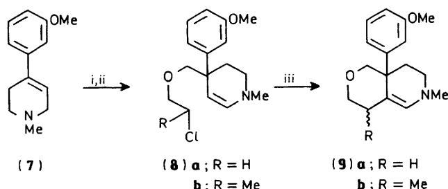
Scheme 1. Reagents: i, BuLi, THF, -20^{\circ}\text{C} ; ii, \text{ClCH}_2\text{OCH}_2\text{CH}_2\text{Cl} ( \text{R} = \text{H} ) or \text{ClCH}_2\text{OCH}_2\text{CH}(\text{Me})\text{Cl} ( \text{R} = \text{Me} ); iii, NaI, MeCN, 85^{\circ}\text{C} ; ( \text{R} = \text{H} ), or 1-methylpyrrolidin-2-one, NaI, 130^{\circ}\text{C} ; ( \text{R} = \text{Me} )
