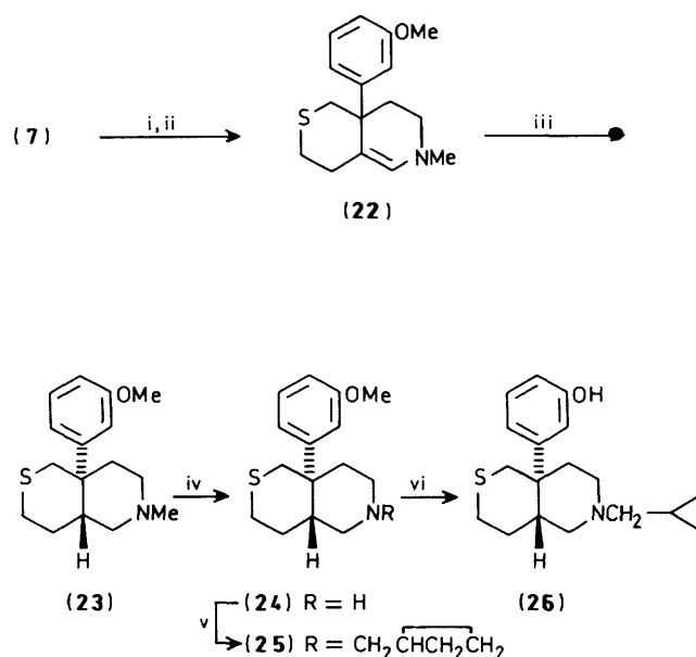
Scheme 2. Reagents: i, (a) BuLi, THF, -20^{\circ}\text{C} ; (b) ClCH 2 SCH 2 CH 2 Cl, -70^{\circ}\text{C} ; ii, NaI, CH 3 CN, heat; iii, (a) MeSO 3 H, MeOH, -65^{\circ}\text{C} ; NaBH 4 ; iv, (a) ClCO 2 Ph, Bu i 3 N, ClCH 2 CH 2 Cl, (b) KOH, EtOH; v, CH 2 CH 2 CH=CH 2 Br, NaHCO 3 , DMF; vi, LiSMc, DMF
