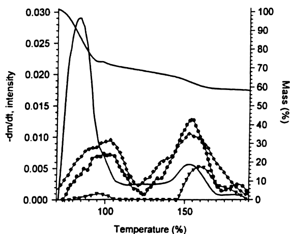
Fig. 3. Comparison of TG, DTG and ion intensity curves of \text{N}_2 , \text{NO}^+ and \text{N}_2\text{O} ( m/z 28: \bullet -, m/z 30: \blacktriangledown - and m/z 44: \blacklozenge -, respectively). (Ion intensity curves are in arbitrary scales).
