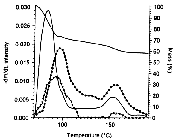
Fig. 1. Comparison of TG, DTG and ion intensity curves of H 2 O and O 2 (m/z 18: -●- and m/z 32: -▼-, respectively) during the thermal decomposition of NH 4 MnO 4 . (Ion intensity curves are in arbitrary scales.)
