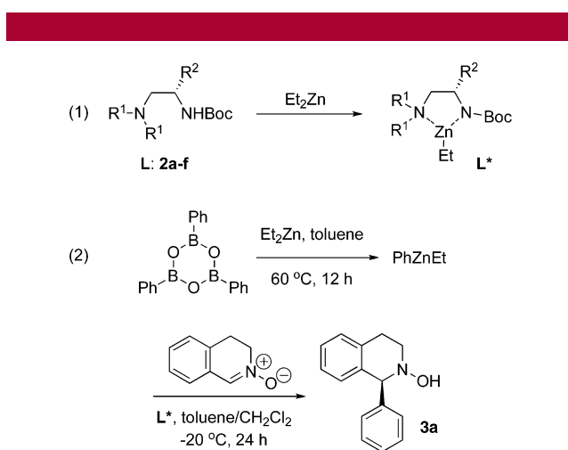
Figure 2. (1) Formation of the active catalyst L* by reaction of ligands 2a–f with Et 2 Zn. (2) L* promoted enantioselective addition of PhZnEt to 3,4-dihydroisoquinoline N -oxide.
