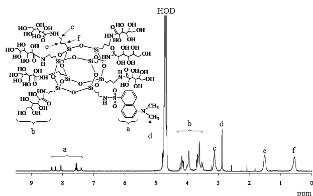
Figure 2. ^1\text{H} NMR spectrum of 3 in \text{D}_2\text{O} .
