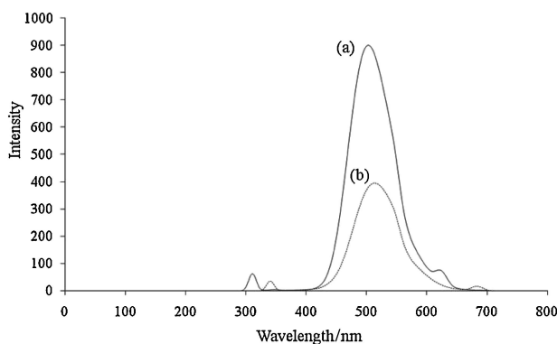
Figure 5. Fluorescence spectra of 3 excited at 310 nm in water (a) and N -butyl-5-(dimethylamino)naphthalene-1-sulfonamide excited at 340 nm in methanol (b); concentrations; 0.90 \times 10^{-4} \text{ mol L}^{-1} .
