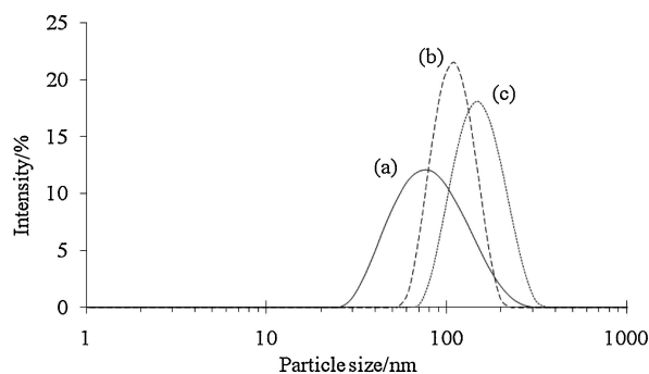
Figure 4. DLS profiles of aqueous dispersions of 3 in various concentrations; 1.0 \times 10^{-4} (a), 1.0 \times 10^{-3} (b), and 2.0 \times 10^{-3} (c) \text{mol L}^{-1} .
