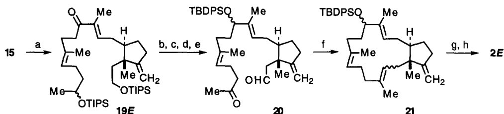
Scheme 4. a) \text{KN}(\text{TMS})_2 , dibenzo-18-crown-6, toluene, r. t., 2 h, then 10 , 0.5 h (84%; 19E/19Z = 86/14); b) DIBAH, toluene, 0 °C (88%); c) TBDPSCl, imidazole, DMF, r. t., 1 day (95%); d) n\text{-Bu}_4\text{NF} , THF, 25 °C, 15 h (86%); e) (\text{COCl})_2 , DMSO, \text{CH}_2\text{Cl}_2 , -60 °C, 2 h, then \text{NEt}_3 (80%); f) \text{TiCl}_3 , Zn-Cu, DME, 80 °C, then addition of 20 via syringe pump over 24 h (54%); g) n\text{-Bu}_4\text{NF} , THF, reflux, 24 h (100%); h) n\text{-Pr}_4\text{NRuO}_4 , NMO, 4 Å molecular sieves, \text{CH}_2\text{Cl}_2 , r. t., 2 h (94%; 2E/2Z = 64/36).
