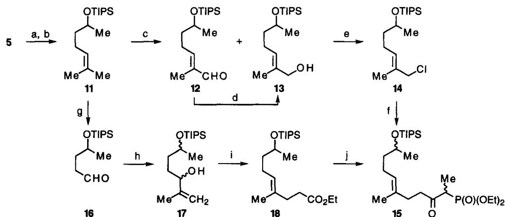
Scheme 3. a) \text{LiAlH}_4 , \text{Et}_2\text{O} , 0^\circ\text{C} , 1 h (100%); b) \text{TIPSCl} , imidazole, DMF, r. t., 8 h (100%); c) \text{SeO}_2 , t - \text{BuO}_2\text{H} , salicylic acid, \text{CH}_2\text{Cl}_2 , r. t., 2.5 days; d) \text{NaBH}_4 , \text{EtOH} , 0^\circ\text{C} , 0.5 h (steps c + d: 61% of 13 ); e) \text{MsCl} , \text{LiCl} , collidine, DMF, 0^\circ\text{C} , 2 h (96%); f) \text{LiCH}_2\text{C}(\text{O})\text{C}(\text{Me})\text{NaP}(\text{O})(\text{OEt})_2 , THF, 0^\circ\text{C} (56%); g) \text{O}_3 , \text{CH}_2\text{Cl}_2 , then \text{Me}_2\text{S} , 12 h (100%); h) \text{CH}_2=\text{C}(\text{Me})\text{MgBr} , THF, r. t., 0.5 h (94%); i) \text{MeC}(\text{OEt})_3 , \text{EtCO}_2\text{H} (0.06 equiv.), 140^\circ\text{C} , 1.5 h (89%); j) \text{MeCHLiP}(\text{O})(\text{OEt})_2 , THF, -78^\circ\text{C} , 15 min. (94%).
