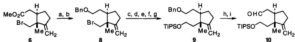
Scheme 2. a) \text{LiAlH}_4 , \text{Et}_2\text{O} , -60^\circ\text{C} , 1.5 h (94%); b) \text{KN}(\text{TMS})_2 , THF, 0^\circ\text{C} , 0.5 h, then \text{BnBr} (93%); c) \text{NaCN} , \text{DME:HMPA} 3:2, 100^\circ\text{C} , 2 days (93%); d) \text{DIBALH} , toluene, 0^\circ\text{C} , 0.5 h; e) \text{H}_3\text{O}^+ (steps d + e: 70%); f) \text{LiAlH}_4 , \text{Et}_2\text{O} , 0^\circ\text{C} , 0.5 h (92%); g) \text{TIPSCl} , imidazole, DMF, 12 h (97%); h) \text{Li} , \text{EtNH}_2 , THF, -78^\circ\text{C} , 1.5 h (97%); i) (\text{COCl})_2 , DMSO, \text{CH}_2\text{Cl}_2 , -60^\circ\text{C} , 4 h, then \text{NEt}_3 (98%).
