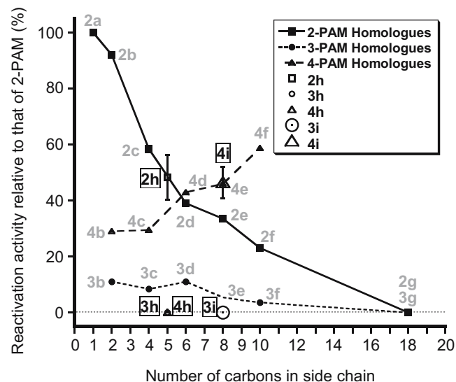
Fig. 4. Relative AChE reactivation activities of PAM analogues with branched alkyl side chains to 2-PAM.
