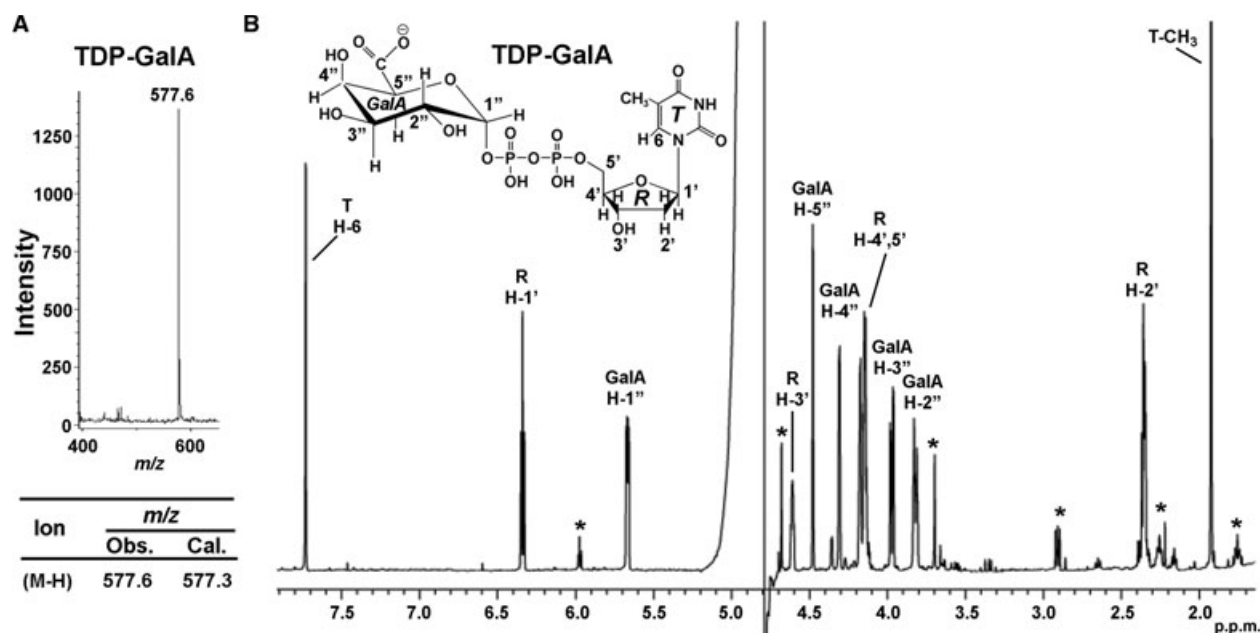
Fig. 6. ^1\text{H} -NMR spectroscopic and MALDI-TOF analyses of BcUGlCAE reaction products indicates the formation of TDP- \alpha -D-galacturonic acid. (A) The HPLC peaks (Fig. 5C, panels 2–4) corresponding to the product formed by BcUGlCAE were collected and analyzed by MALDI-TOF. (B) ^1\text{H} -NMR spectroscopy at 600 MHz of the HPLC peak from Fig. 5C (panel 3). The assignments of each proton are indicated on the spectrum: peaks from protons on the thymidine (T) ring are indicated by H, the ribose (R) protons are indicated by H', and the GalA (G) protons are indicated by H''. The peaks marked by an asterisk (*) are resonances from impurities.
