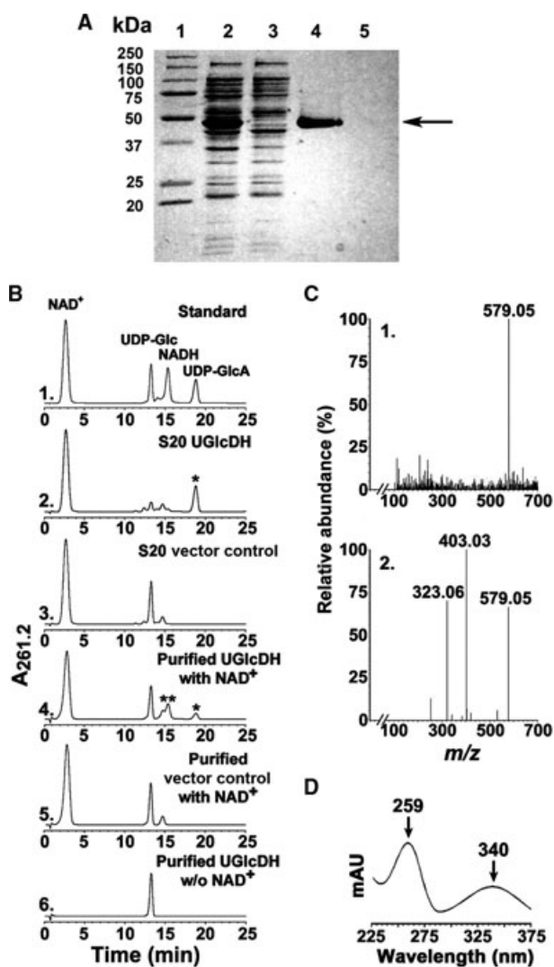
Fig. 2. Expression and characterization of recombinant of BcUGlcDH. (A) SDS/PAGE of total soluble protein isolated from E. coli cells expressing UGlcDH (lane 2), negative vector control (lane 3) and of column-purified UGlcDH or control (lanes 4 and 5, respectively). An arrow points to the purified protein. (B) High-performance anion-exchange chromatography of the products formed by UGlcDH. Purified recombinant UGlcDH was reacted with UDP-Glc for 30 min in the presence (panel 4) or absence (panel 6) of \text{NAD}^+ . The corresponding column-purified protein isolated from cells expressing the control vector was reacted with UDP-Glc and \text{NAD}^+ for 30 min (panel 5) as a control. The reaction products were separated on a Q15 anion-exchange column. The distinct UDP-sugar peak marked by an asterisk (panels 2 and 4 with a retention time of 18.8 min) was collected and characterized by mass spectrometry and ^1\text{H} -NMR spectroscopy. The activity of total soluble protein (denoted S20) isolated from cells expressing recombinant BcUGlcDH (panel 2) or vector control (panel 3) is also shown. (C) Analysis of BcUGlcDH enzymatic product by MS operated in the negative ion mode. The HPLC peak (panel 2B or 4B, *) was collected and directly infused to ESI-MS. The spectrum of the full MS molecular ions (panel 1, m/z of 579.05 for deprotonated [\text{M}-\text{H}]^- ) and of the derived CID-fragments (panel 2, m/z of 323.06 and 403.05) are shown. (D) The peak in panel 4B marked by a double asterisk (**) has major UV absorbance peaks at 259 and 340 nm, the characteristic absorbance signature for NADH.
