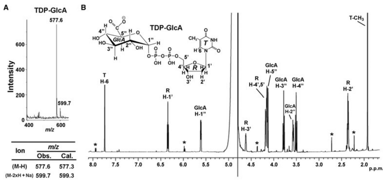
Fig. 4. BcUGlcDH can convert TDP-Glc to TDP-GlcA as determined by MALDI and NMR. (A) MALDI-MS analysis: negative-ion MALDI mass spectra were recorded using a Microflex LT mass spectrometer (Bruker Daltonik, Bremen, Germany). Aqueous samples (1 \mu L) of 1 mM TDP-GlcA (produced from the dehydrogenase reaction with TDP-Glc/ \text{NAD}^+ and collected by HPLC) were mixed with an equal volume of matrix solution (1 \mu\text{g}\cdot\mu\text{L}^{-1} 2,5-dihydroxybenzoic acid in 50% methanol) and dried on the plate. Spectra from 500 laser ( \text{N}_2 ; 337 nm) shots were summed to generate a mass spectrum. The ion mass, calculated (abbr. Cal.) or observed (abbr. Obs.), are listed below the spectrum. (B) ^1\text{H} -NMR spectroscopy at 600 MHz of the HPLC collected peak after reaction of BcUGlcDH with TDP-Glc and \text{NAD}^+ . The assignments of each proton are indicated on the spectrum: peaks from protons on the thymidine (T) ring are indicated by H, the ribose (R) protons are indicated by H', and the GlcA (G) protons are indicated by H''. The peaks marked by an asterisk (*) are resonances from impurities.
